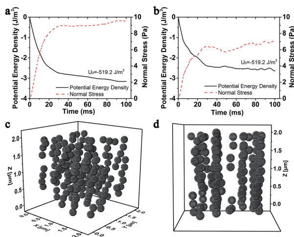
Fig. 7 (a) Time variation magnetic potential energy density and normal stress curves of 20 wt% MSiNP magnetic fluid at a shear rate of \dot{\gamma} = 10\text{ s}^{-1} and (b) \dot{\gamma} = 40\text{ s}^{-1} . (c) The isometric microstructure diagram and (d) the x -axis microstructure diagram of 20 wt% MSiNP magnetic fluid at a shear rate of \dot{\gamma} = 40\text{ s}^{-1} . The magnetic flux density B = 240 mT.
